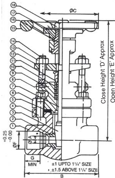
General Arrangement
